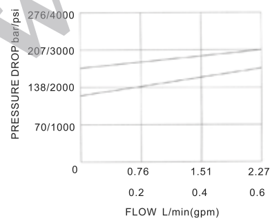
Pressure drop-flow curve 32 cST Oil/45°C
