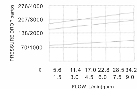
Pressure drop-flow curve 32 cST Oil/45°C
