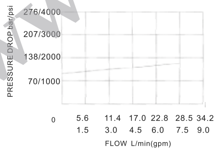
Pressure drop-flow curve 32 cST Oil/45°C
