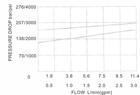
Pressure drop-flow curve 32 cST Oil/45°C
